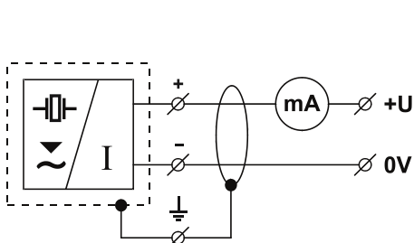
Wiring diagram of the level meter with current output EMKOSONIC-60_--_-I
