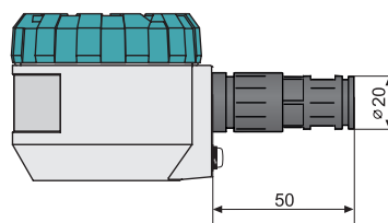
variant EMKOSONIC-60 with protective conductor
