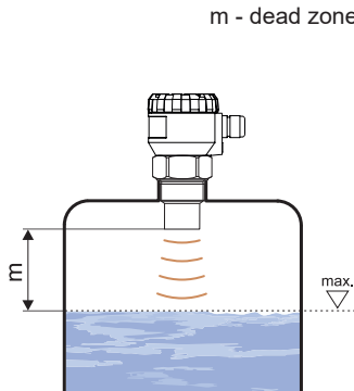
Maximum level distance from EMKOSONIC
