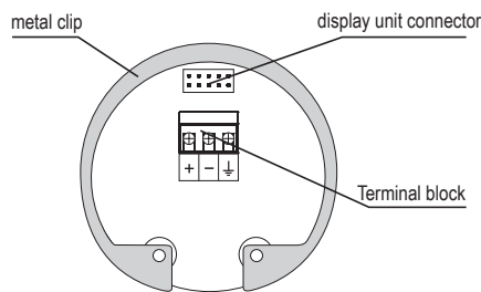
Inside view of screw terminals of the level meter with current output EMKOSONIC-60_--_-I
