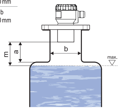
Possible installation through the neck
