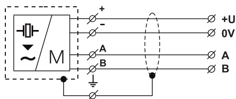
Wiring diagram of the level meter with Modbus EMKOSONIC-60_--_-M
