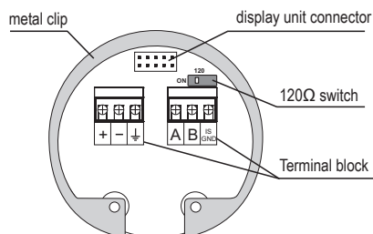
Inside view of screw terminals of the level meter with Modbus EMKOSONIC-60_--_-M
