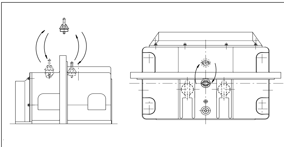
Illustration 1: Assembly device
