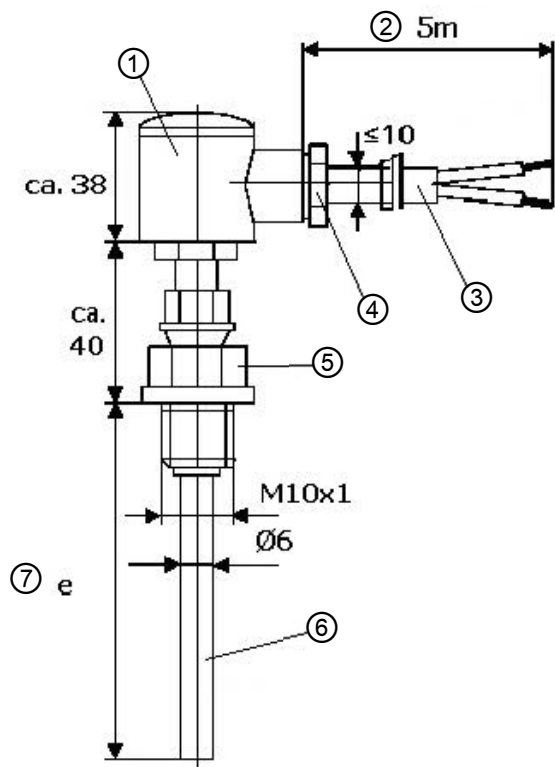
Figure 8: Resistance thermometer
