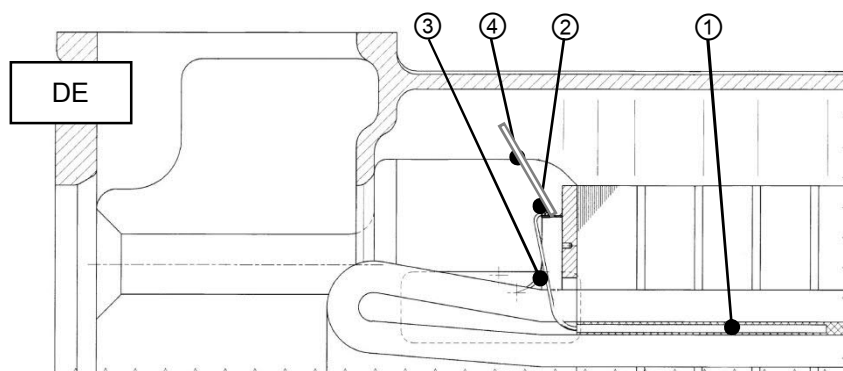
Figure 5: Section B-B
