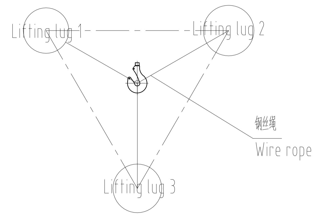
吊具起吊位置示意 Lifting position diagram of spreader
