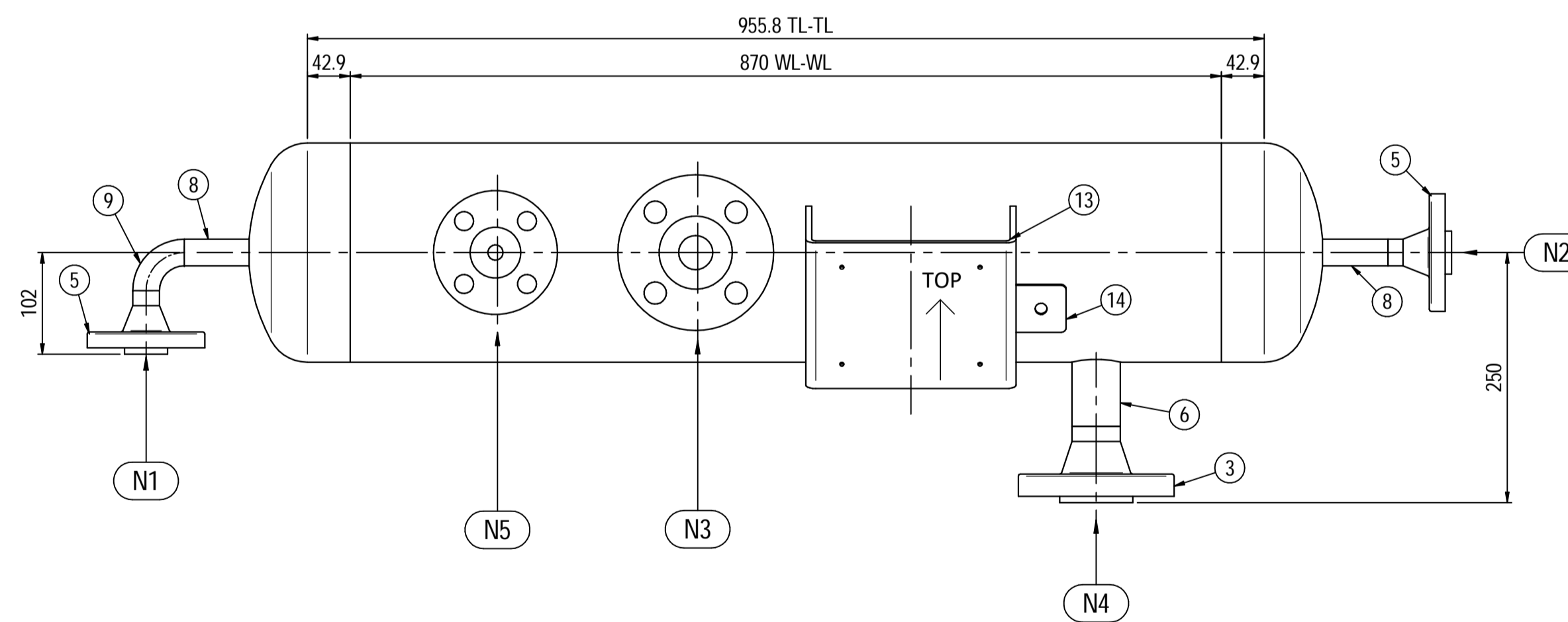
PLAN VIEW
