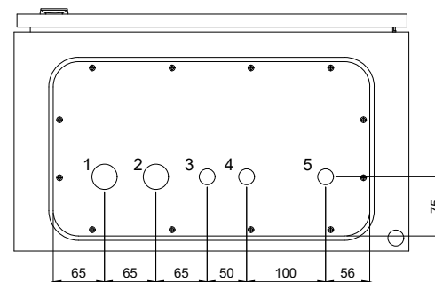
Gland Entry Details
