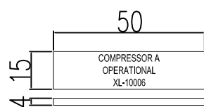
Nameplate for components on panel door (Typical)
